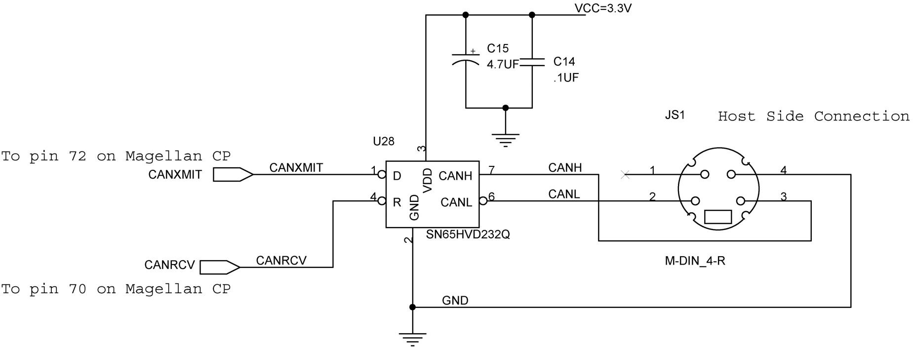
Figure 3.12 - CAN Interface
