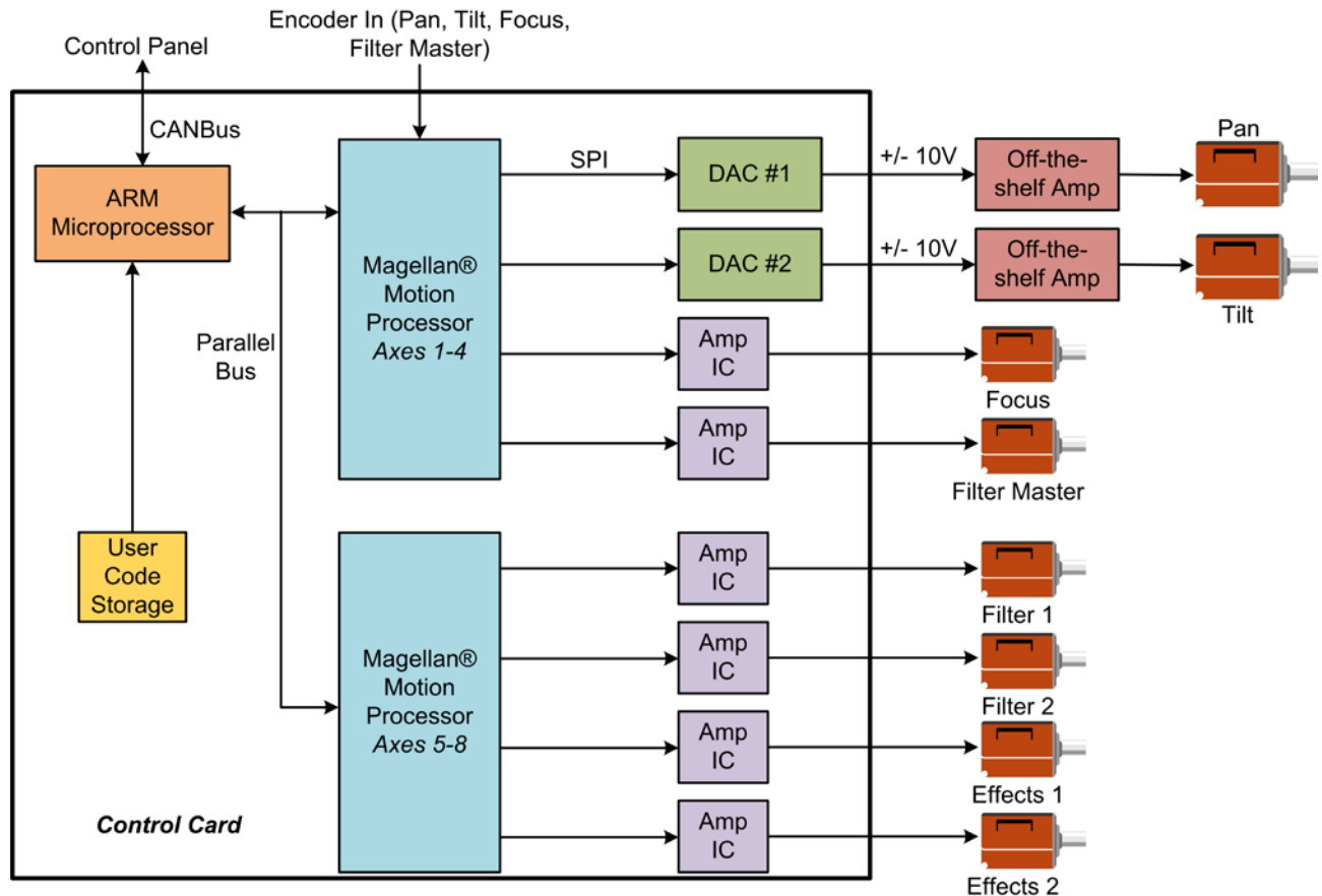
Figure 1: Automated Lighting Solution Controller Card
